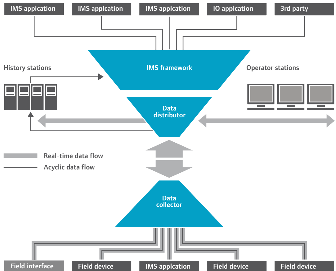
Safety and Automation System Data flow - Real time/acyclic (condition based) through K-PRO
